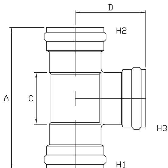
INJECTION MOLDED FITTING (M+)
