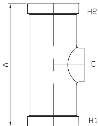
INJECTION MOLDED FITTING (M=) FABRICATED FITTING (F)
